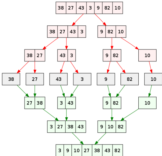
Figura 1: Fonte: https://en.wikipedia.org/wiki/Merge_sort
