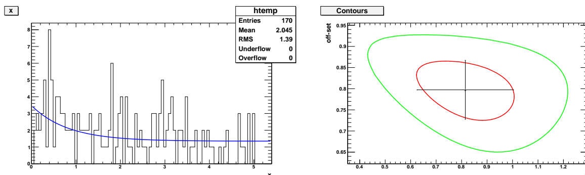
Figure 7.2.: Histogrammed input data with overlaid scaled fit function, and one- and 2- \sigma contour lines from the likelihood fit.
