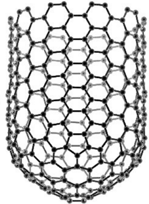
(10,10) tube Nanotubos
